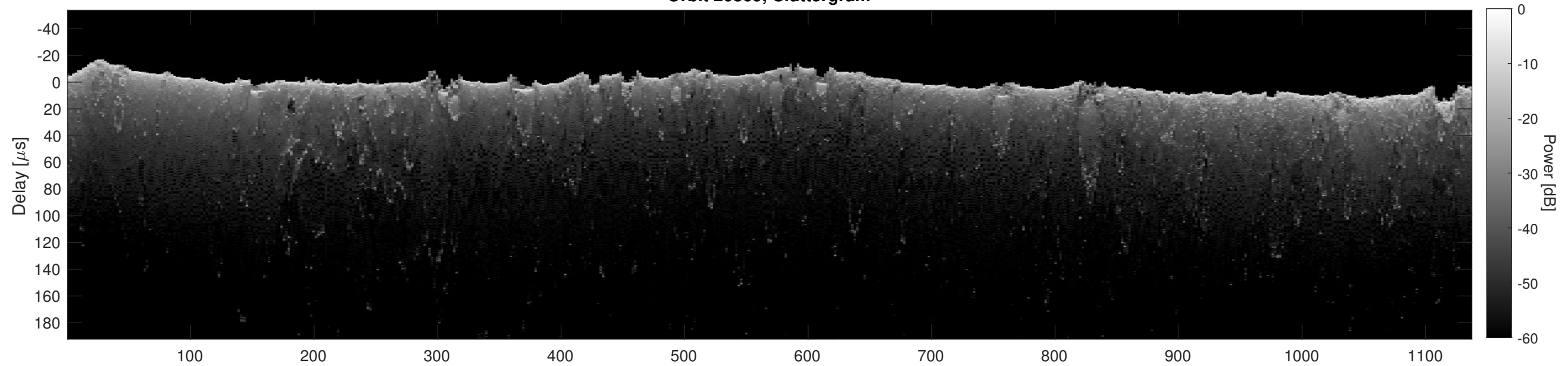
Orbit 20869, Cluttergram
