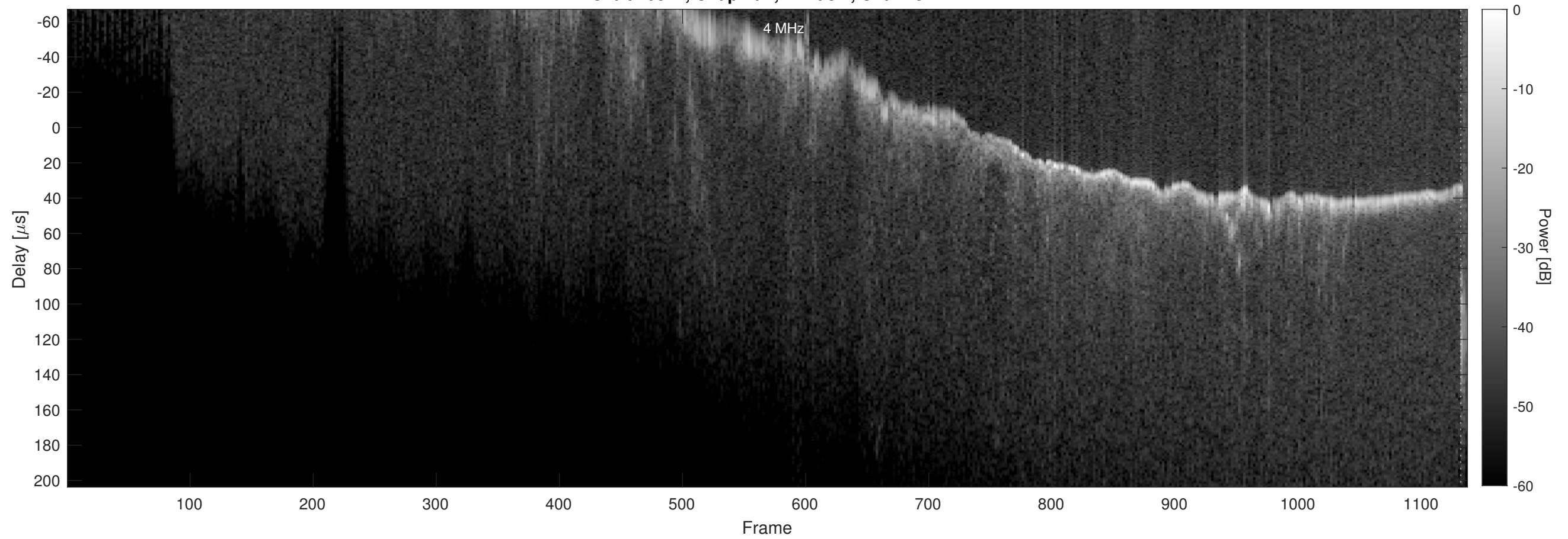
Orbit 20871, Chapman, Window, Channel 2
