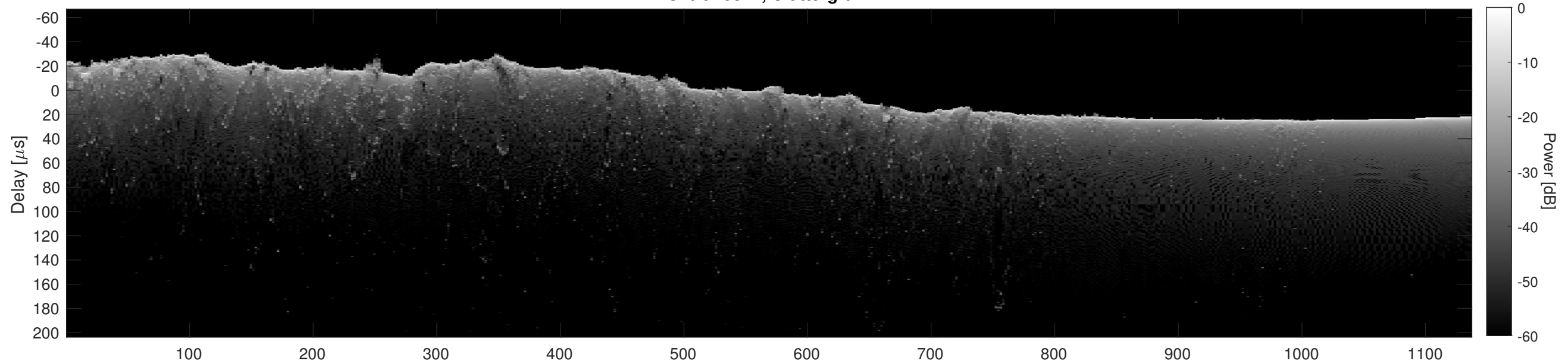
Orbit 20871, Cluttergram
