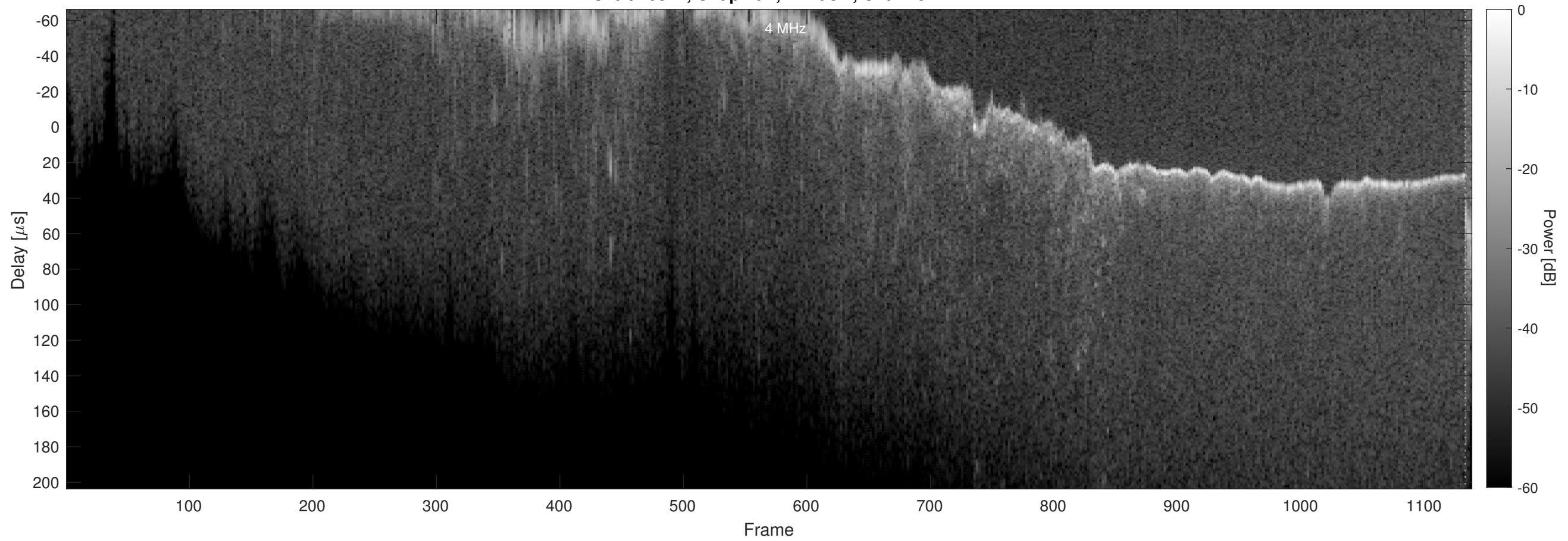
Orbit 20872, Chapman, Window, Channel 2
