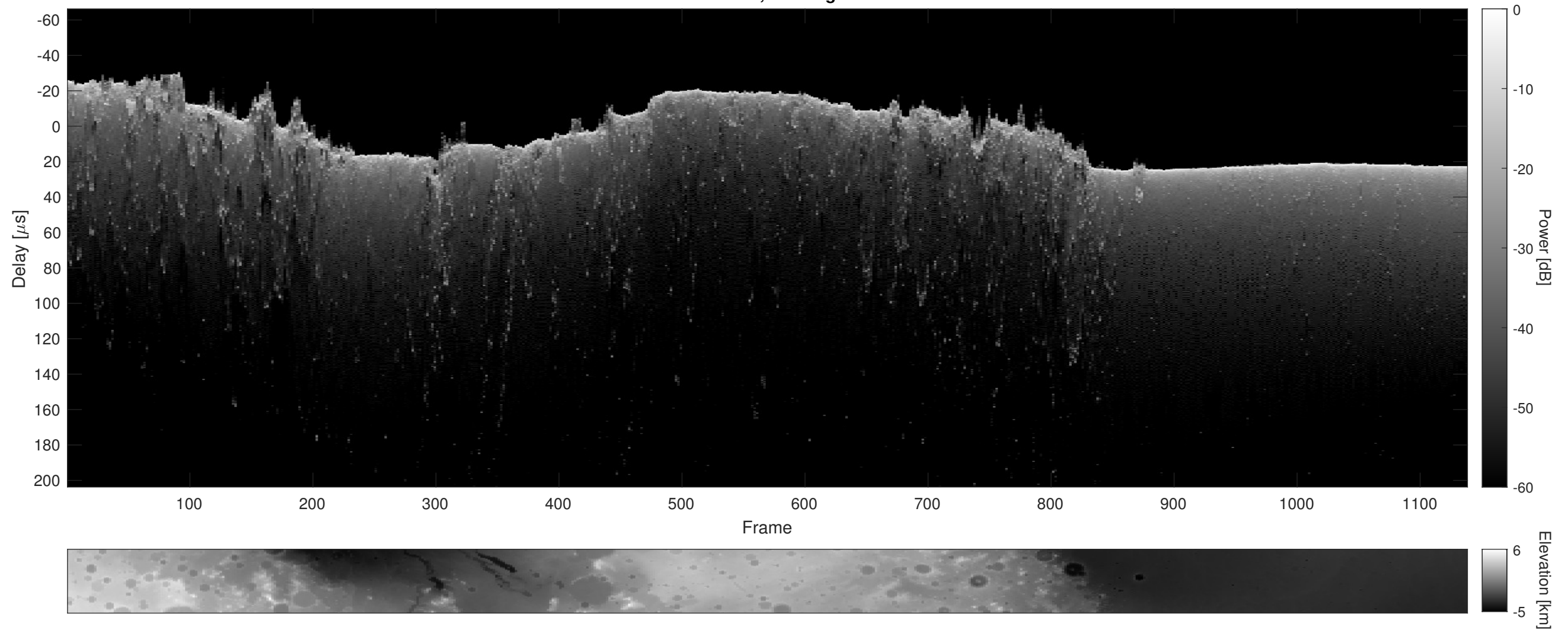
Orbit 20872, Cluttergram
