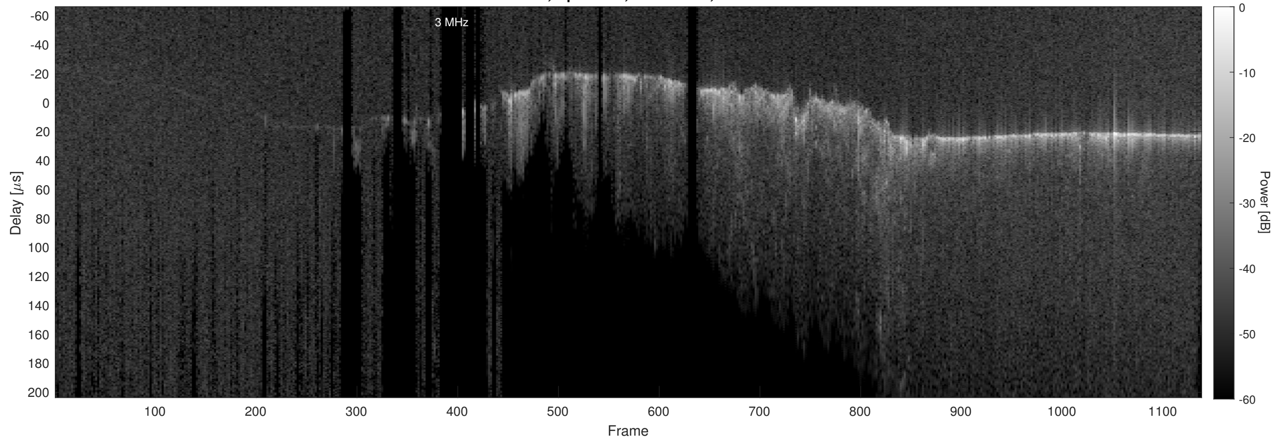
Orbit 20872, Optimized, No Window, Channel 2
