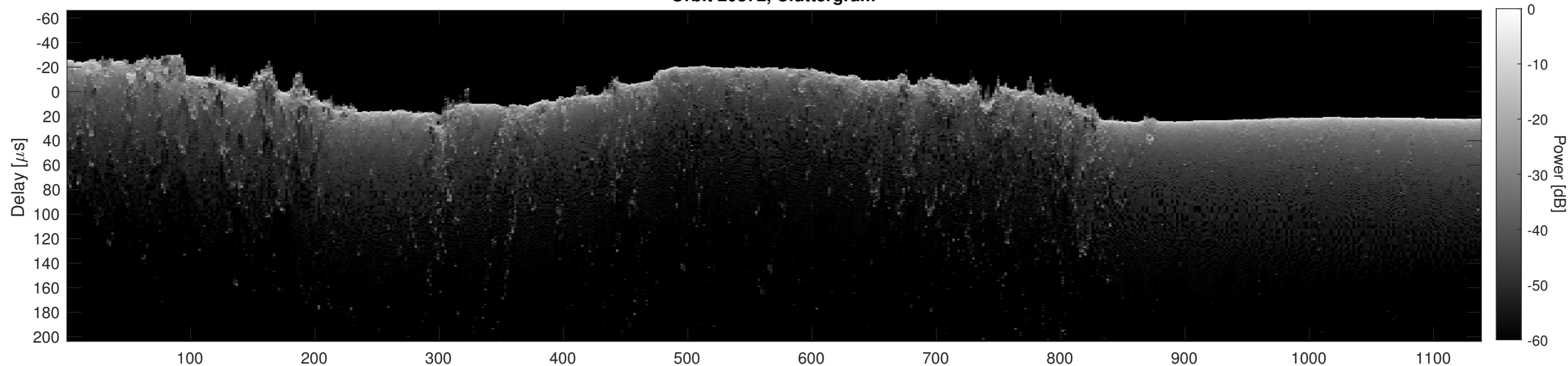
Orbit 20872, Cluttergram
