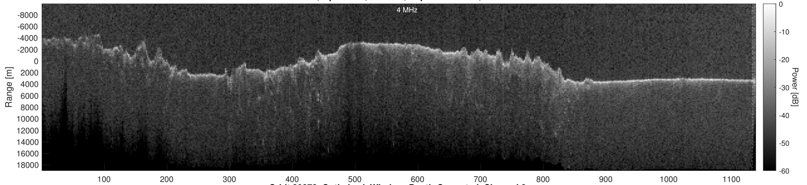
Orbit 20872, Optimized, Window, Depth-Corrected, Channel 2
