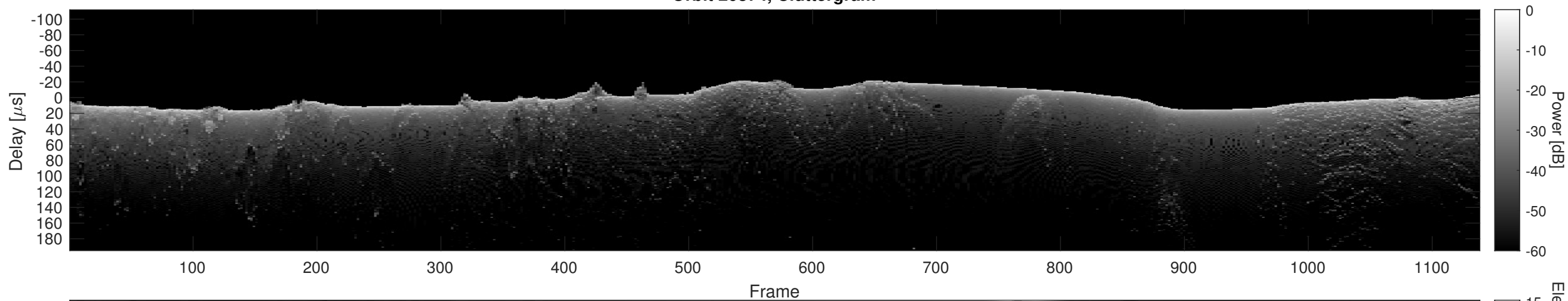
Orbit 20874, Cluttergram
