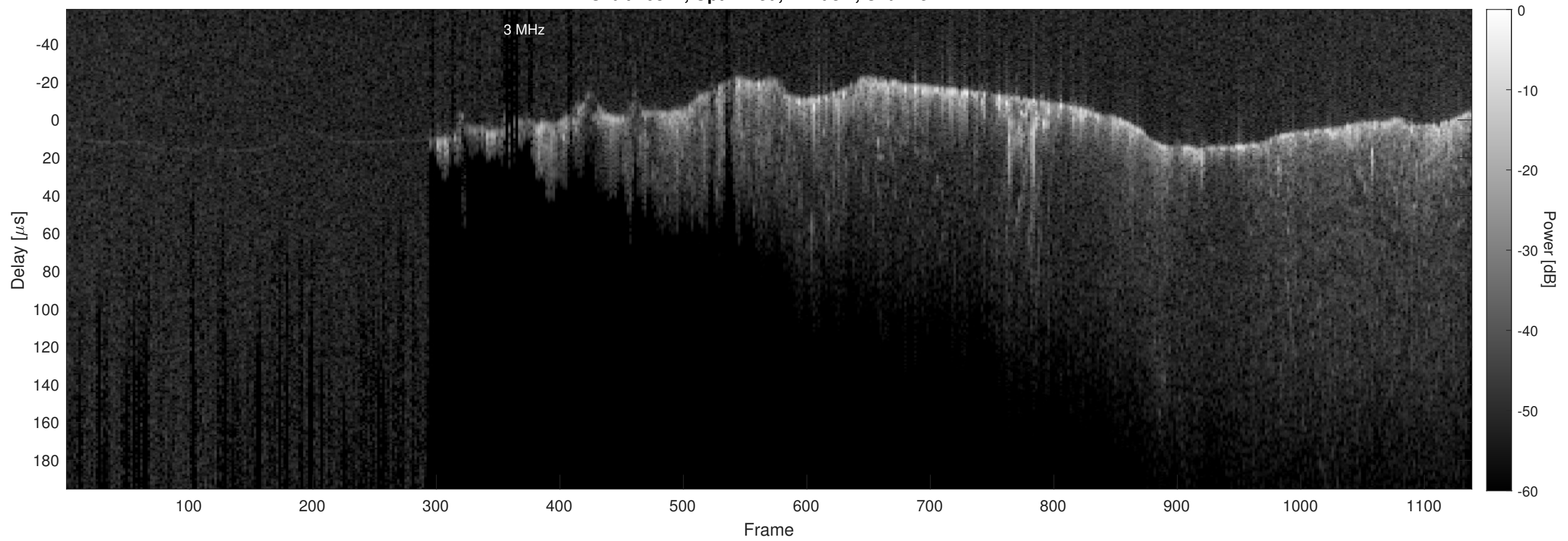
Orbit 20874, Optimized, Window, Channel 2
