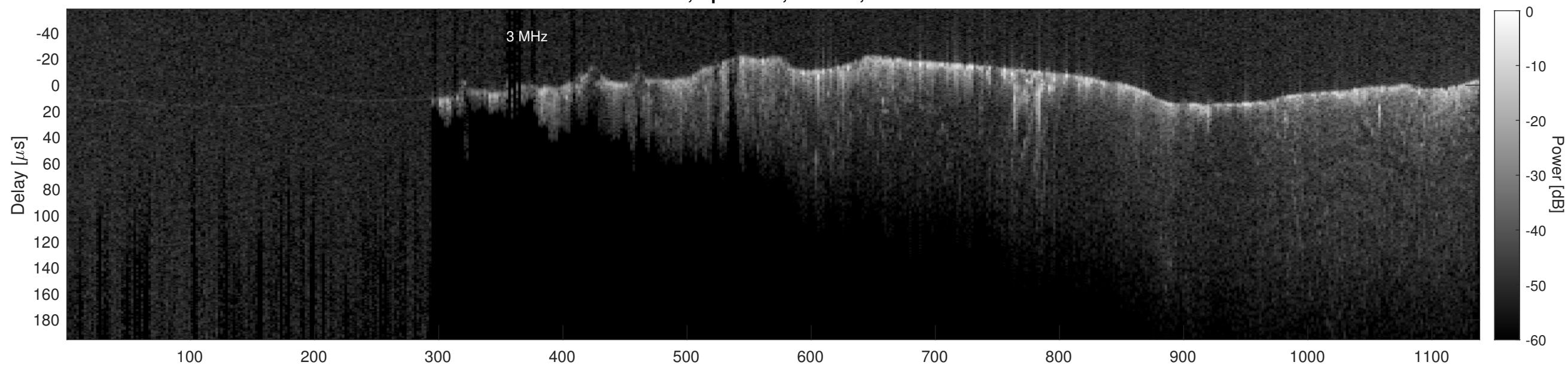
Orbit 20874, Cluttergram
