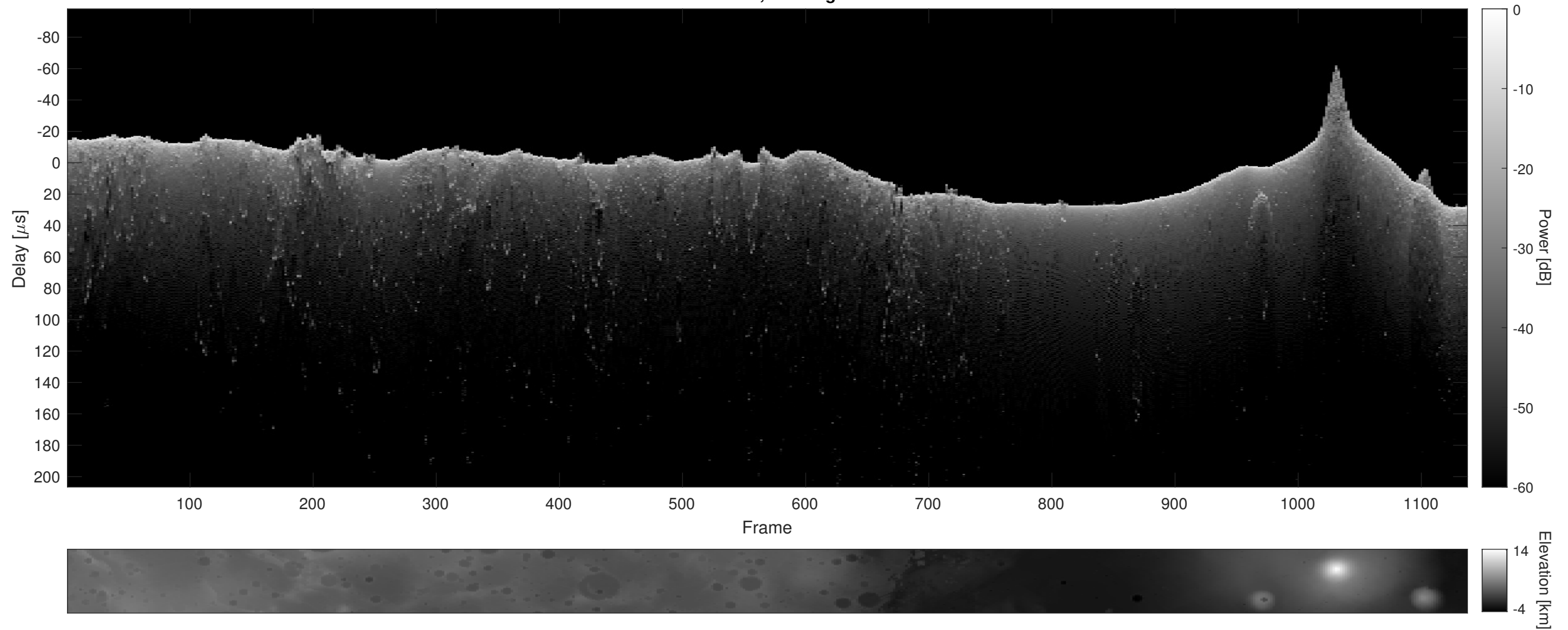
Orbit 20875, Cluttergram
