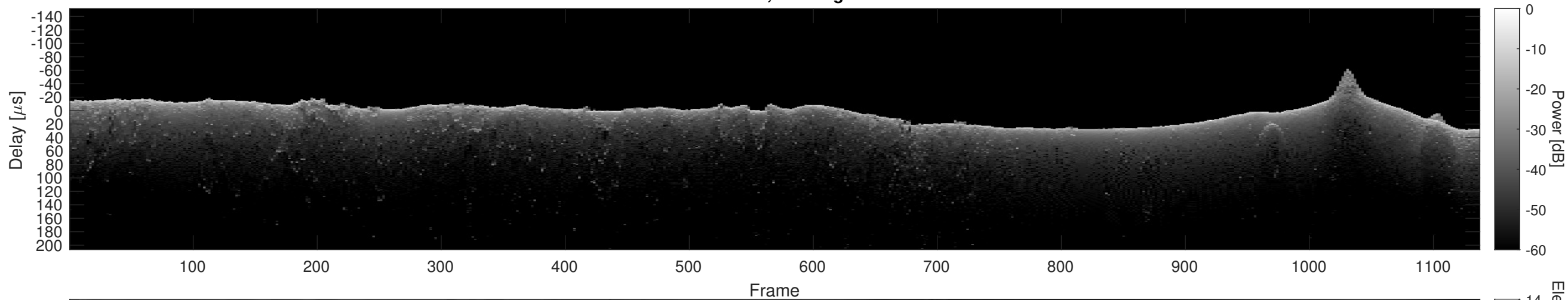
Orbit 20875, Cluttergram
