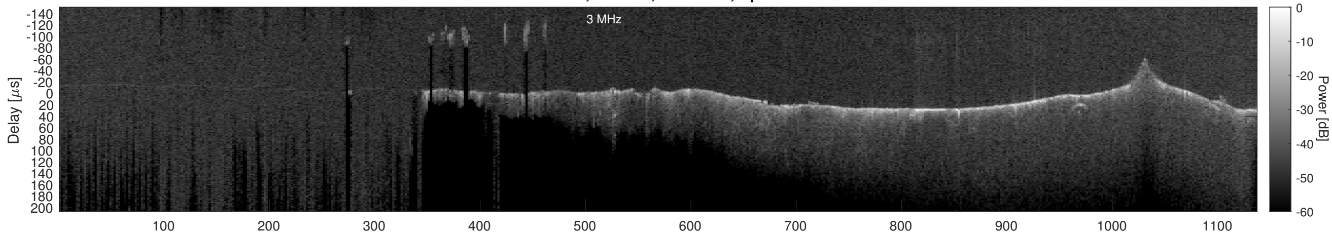
Orbit 20875, Cluttergram
