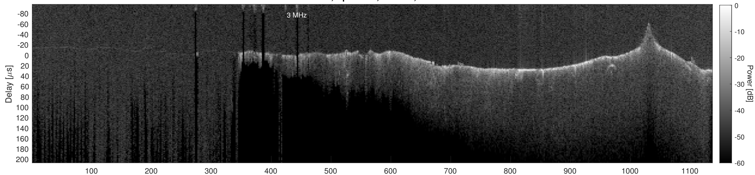
Orbit 20875, Cluttergram
