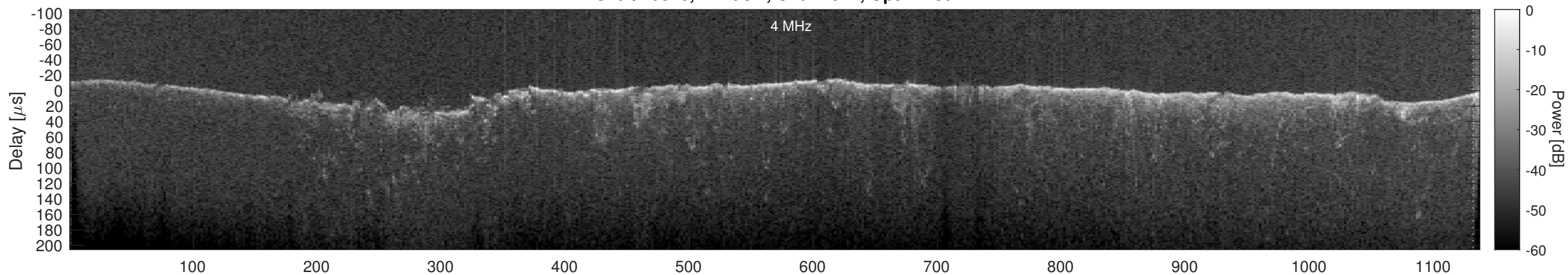
Orbit 20876, Cluttergram
