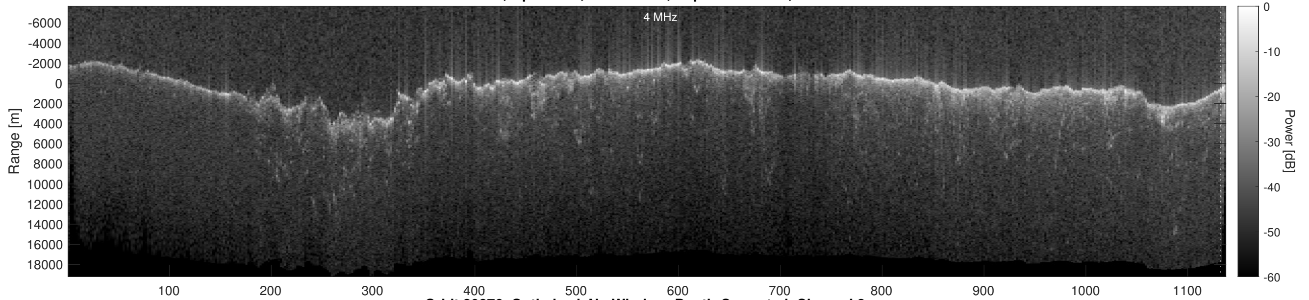
Orbit 20876, Optimized, No Window, Depth-Corrected, Channel 2
