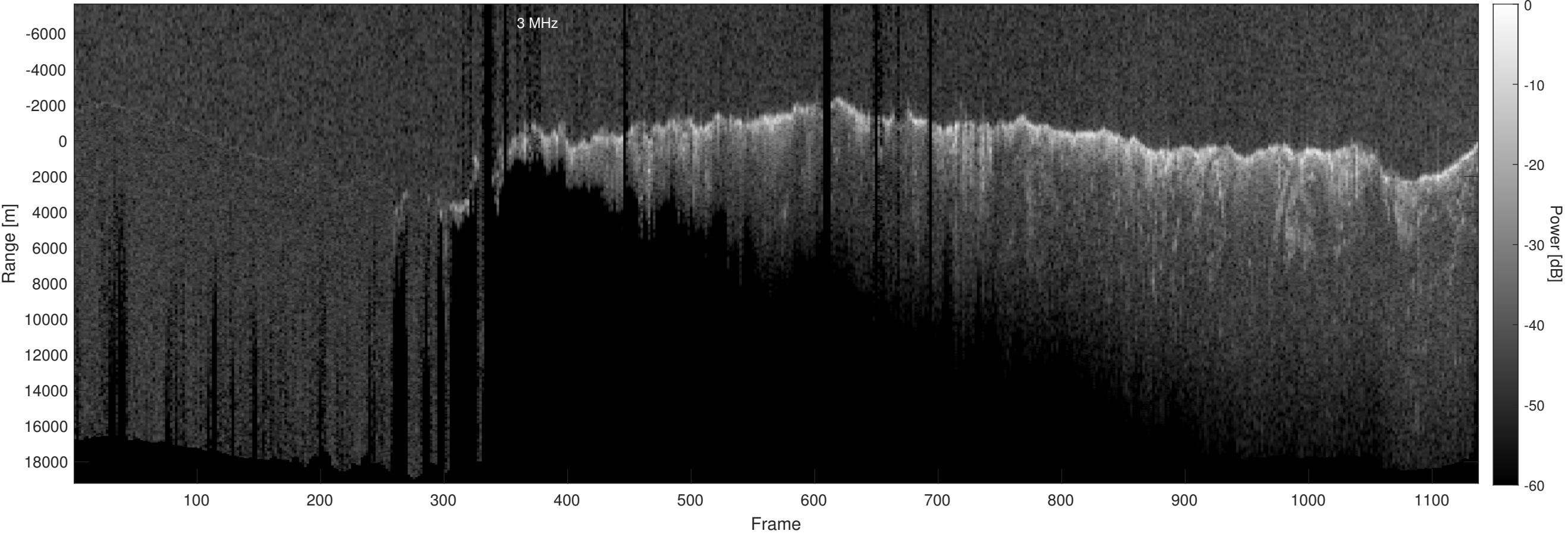
Orbit 20876, Optimized, Window, Depth-Corrected, Channel 2
