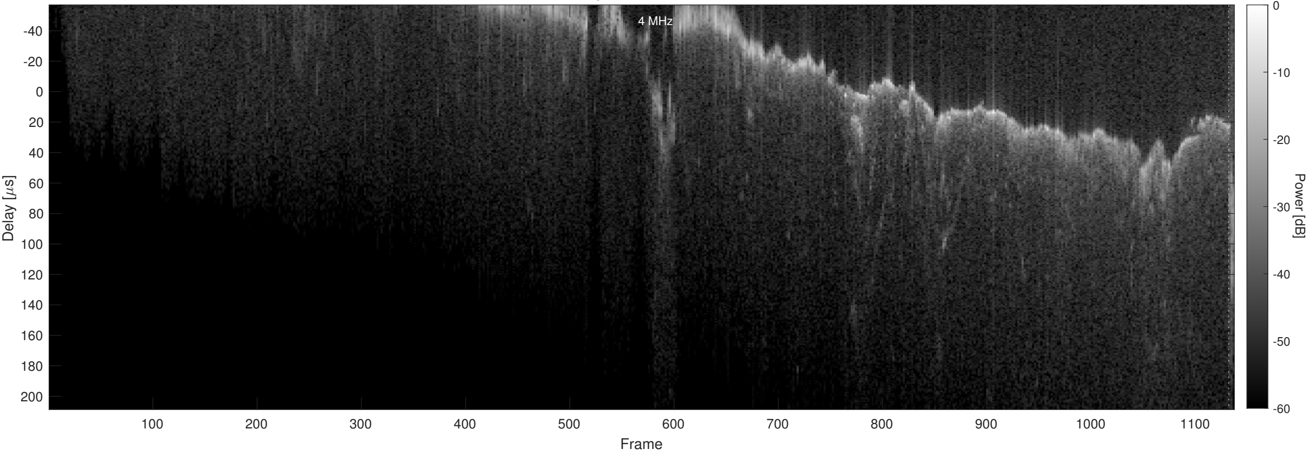
Orbit 20877, Chapman, No Window, Channel 2
