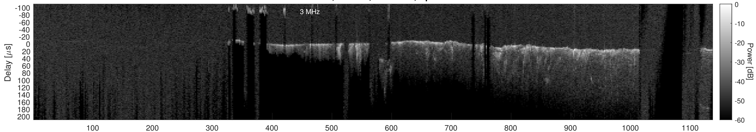
Orbit 20877, Cluttergram
