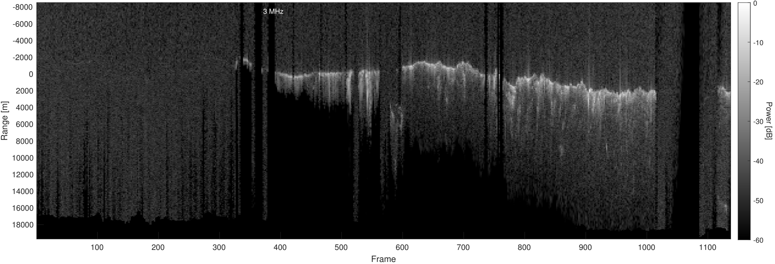
Orbit 20877, Optimized, No Window, Depth-Corrected, Channel 2
