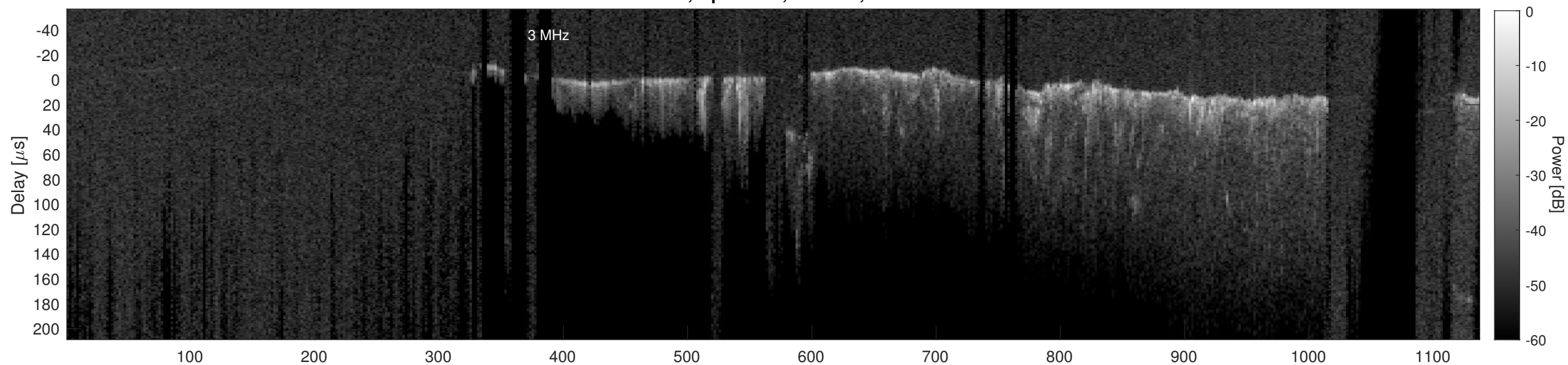
Orbit 20877, Cluttergram
