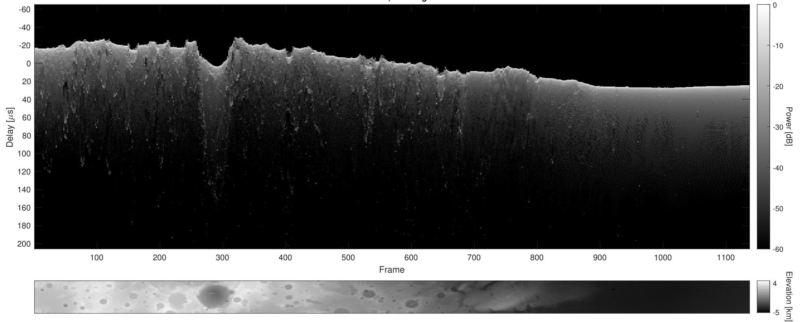
Orbit 20878, Cluttergram
