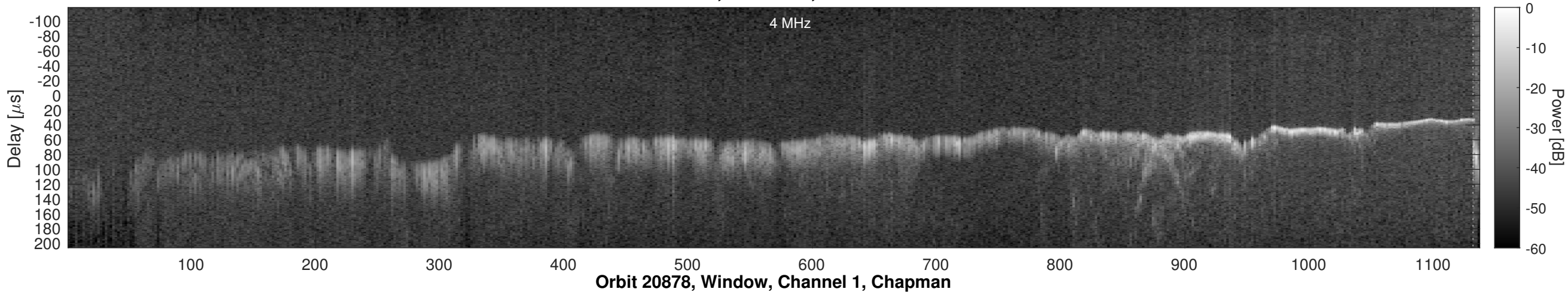
Orbit 20878, Channel 1, Uncorrected
