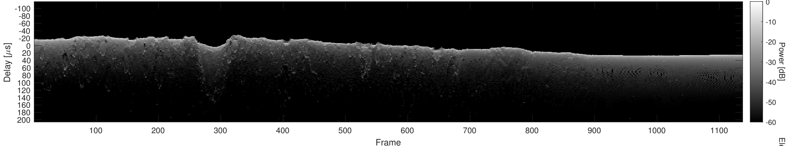
Orbit 20878, Cluttergram
