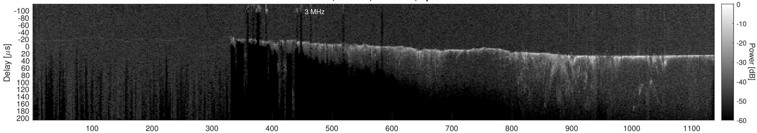
Orbit 20878, Cluttergram
