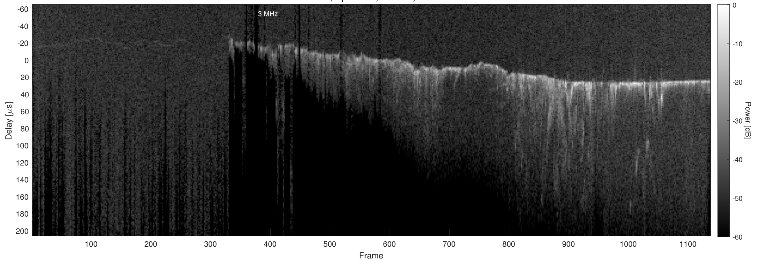
Orbit 20878, Optimized, Window, Channel 2
