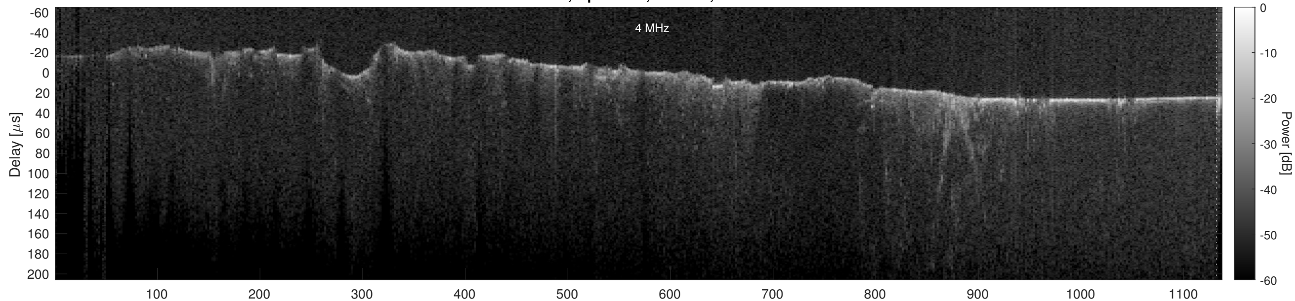
Orbit 20878, Optimized, Window, Channel 2
