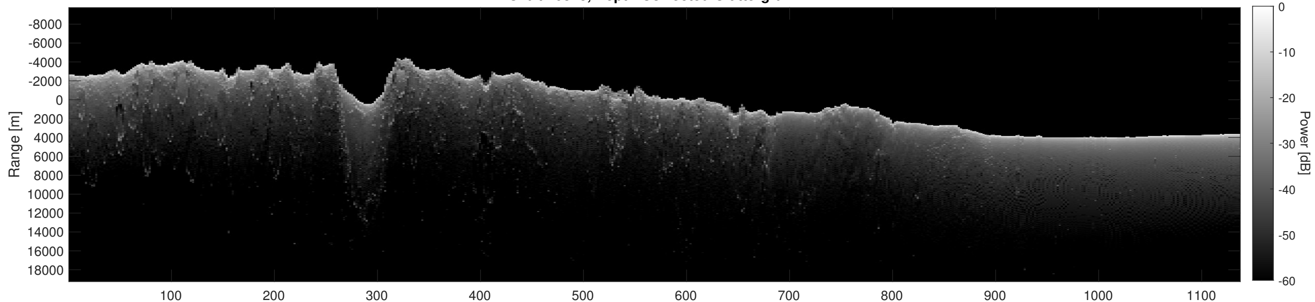
Orbit 20878, Depth-Corrected Cluttergram
