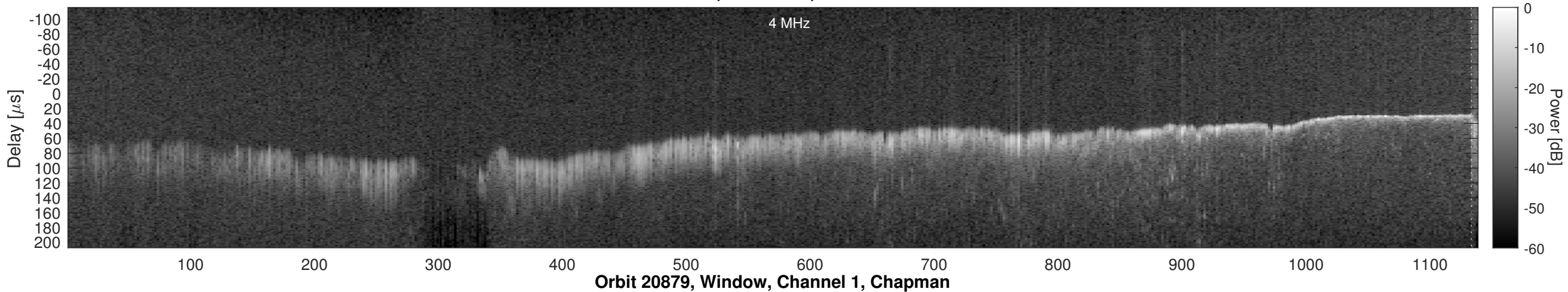
Orbit 20879, Channel 1, Uncorrected
