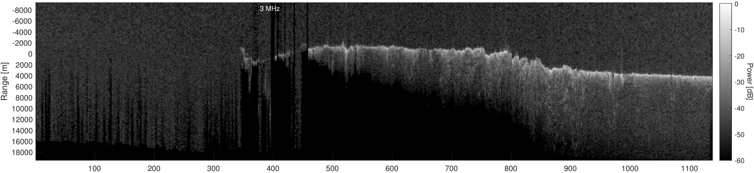
Orbit 20879, Depth-Corrected Cluttergram
