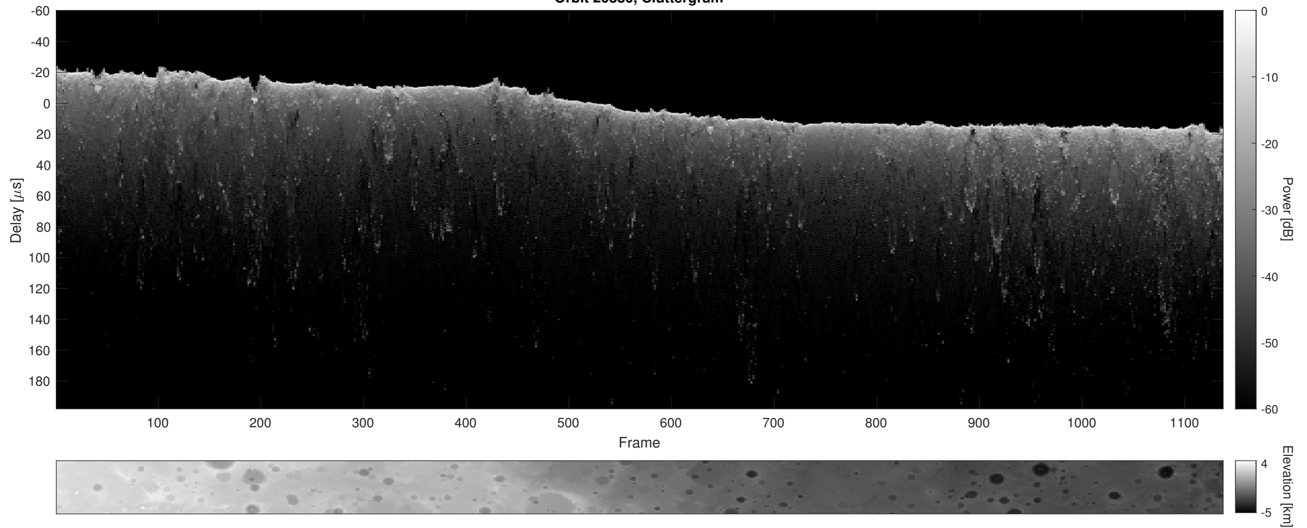
Orbit 20880, Cluttergram
