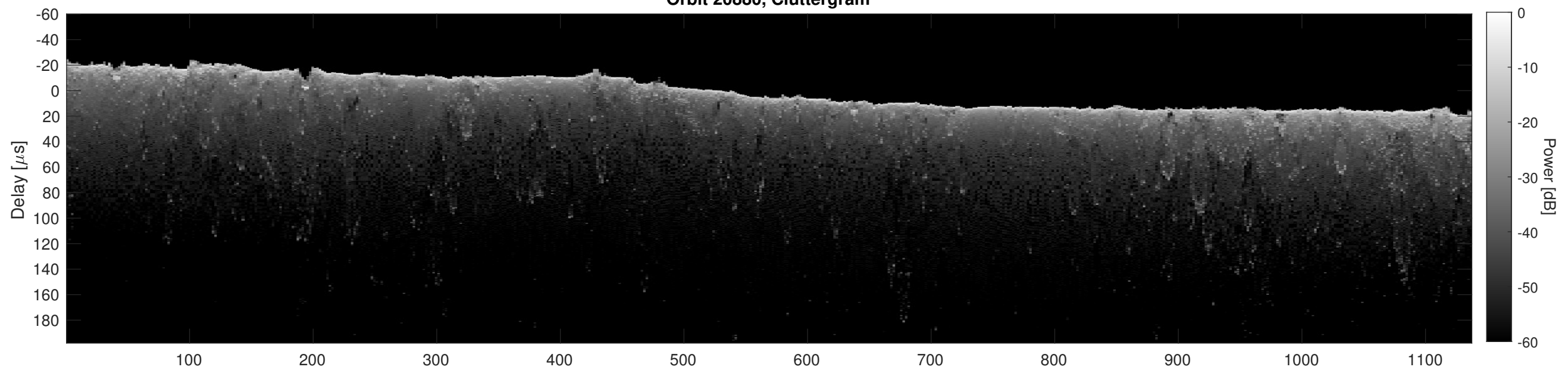
Orbit 20880, Cluttergram
