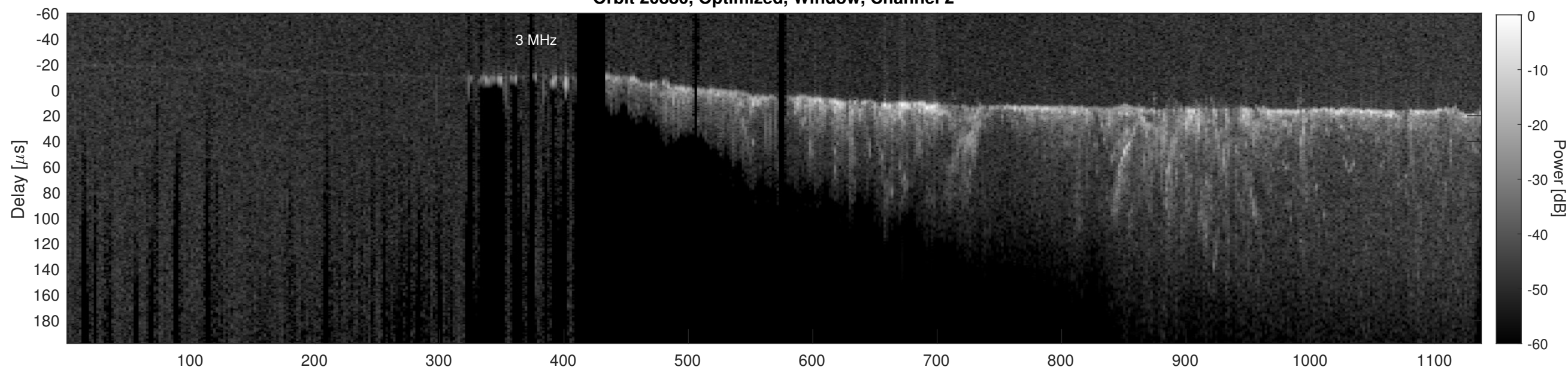
Orbit 20880, Cluttergram
