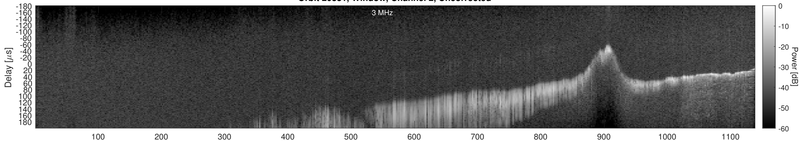
Orbit 20881, Window, Channel 2, Chapman
