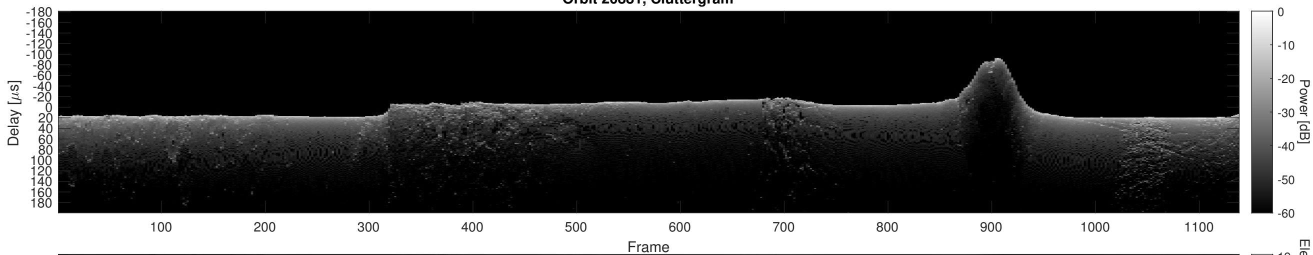
Orbit 20881, Cluttergram
