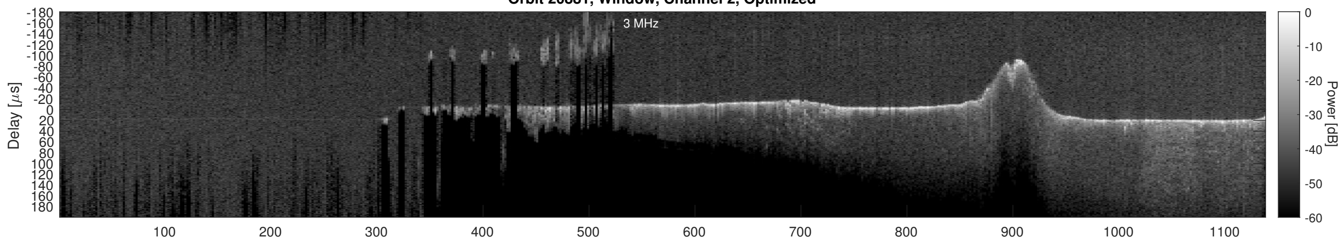
Orbit 20881, Cluttergram
