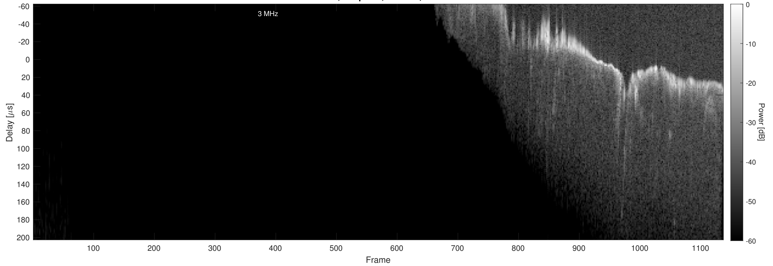
Orbit 20882, Chapman, Window, Channel 2
