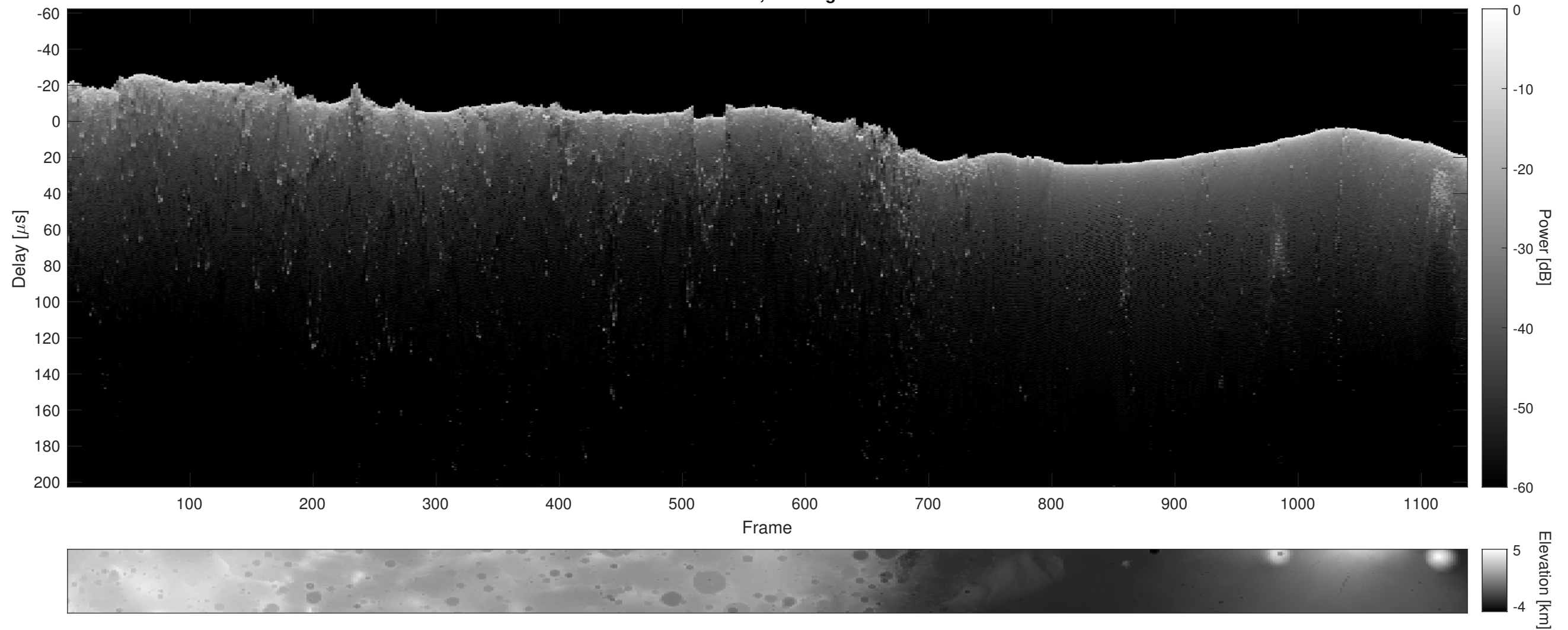
Orbit 20882, Cluttergram
