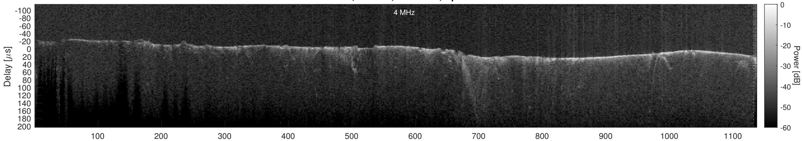
Orbit 20882, Cluttergram
