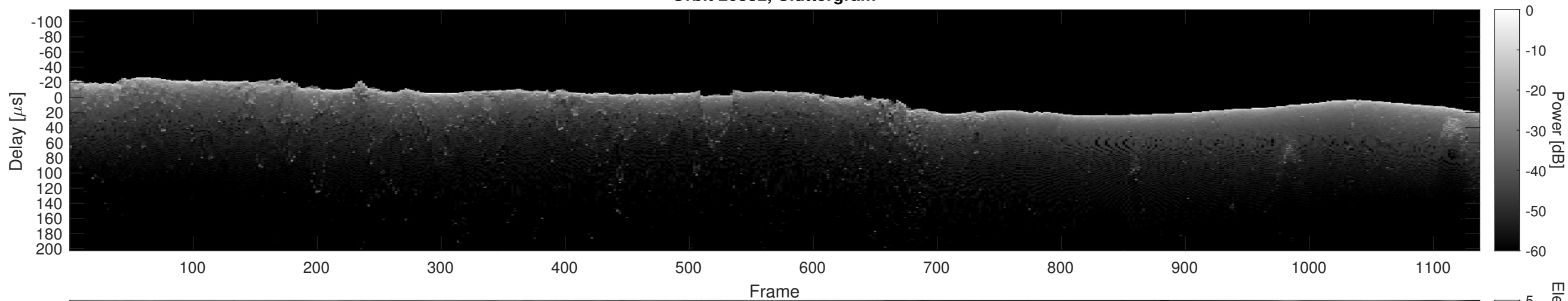
Orbit 20882, Cluttergram
