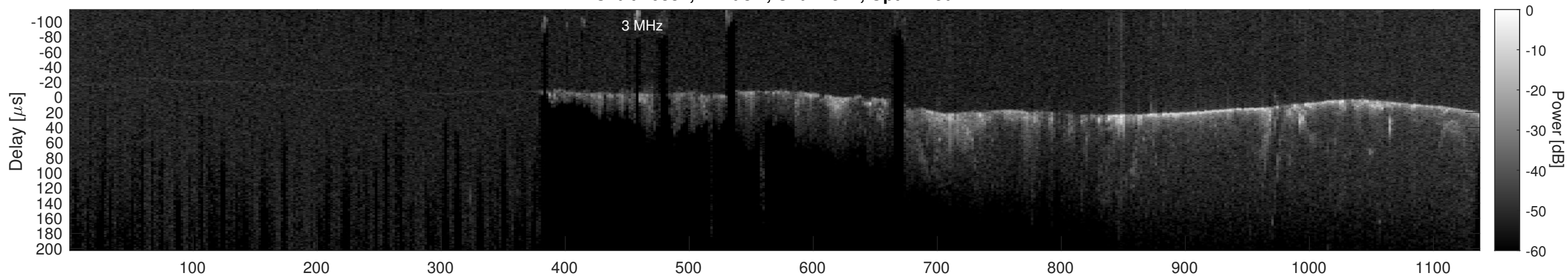
Orbit 20882, Cluttergram
