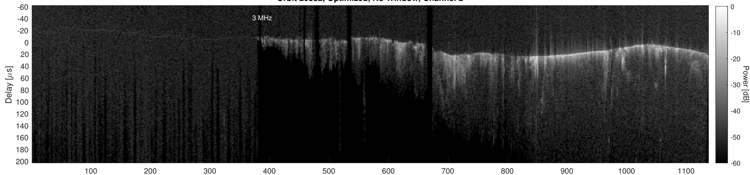
Orbit 20882, Cluttergram
