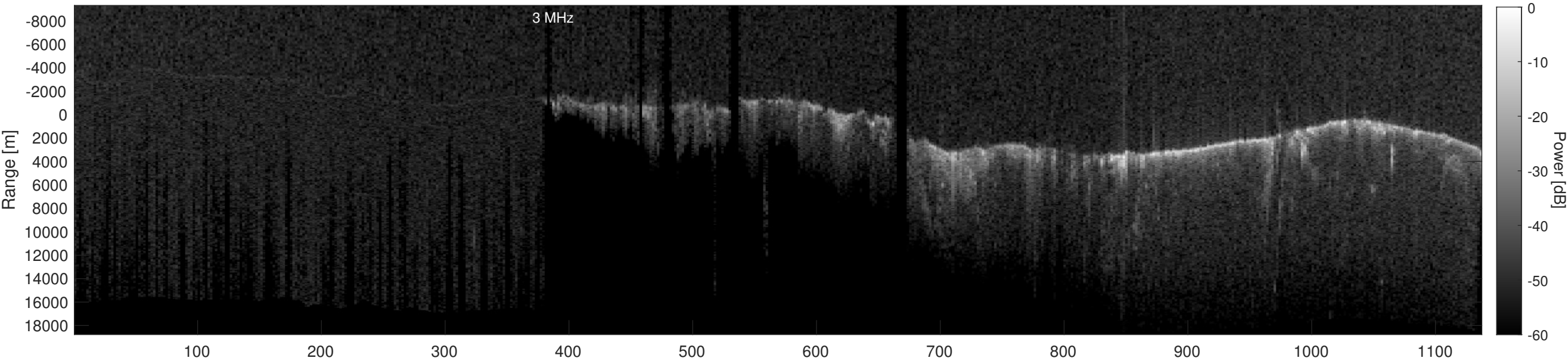
Orbit 20882, Depth-Corrected Cluttergram
