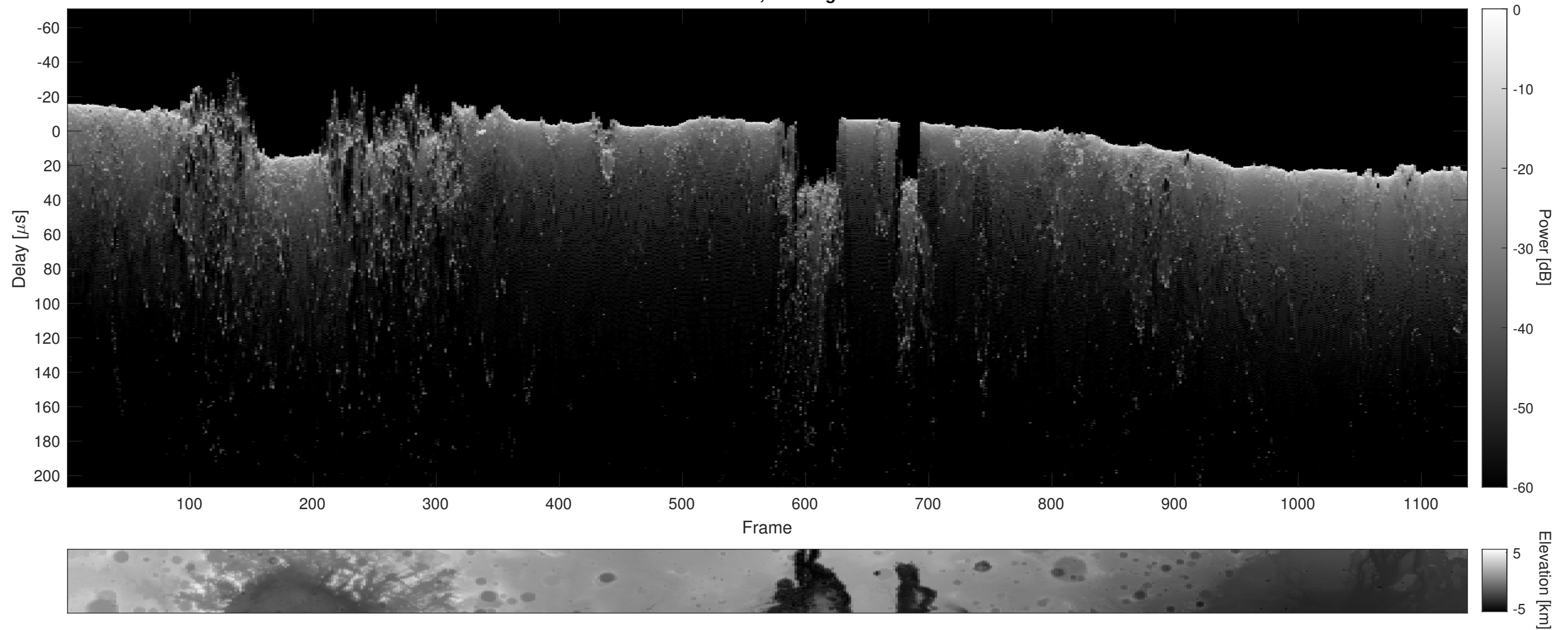
Orbit 20884, Cluttergram
