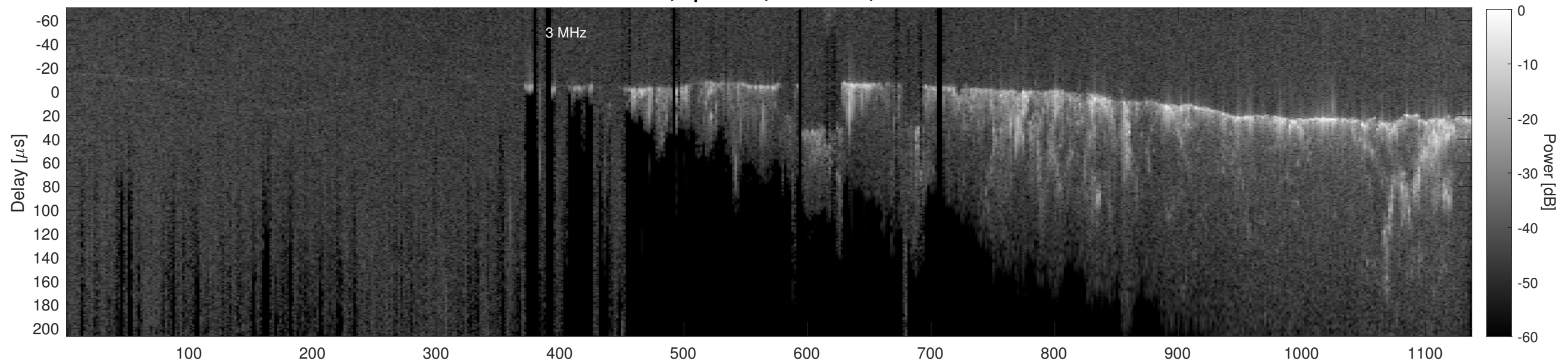
Orbit 20884, Cluttergram
