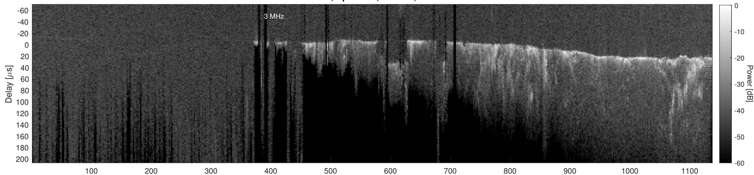
Orbit 20884, Cluttergram
