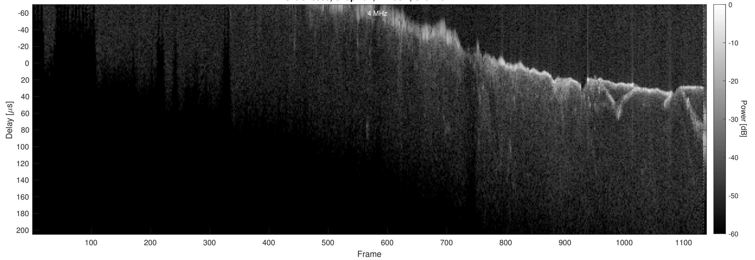
Orbit 20885, Chapman, Window, Channel 2
