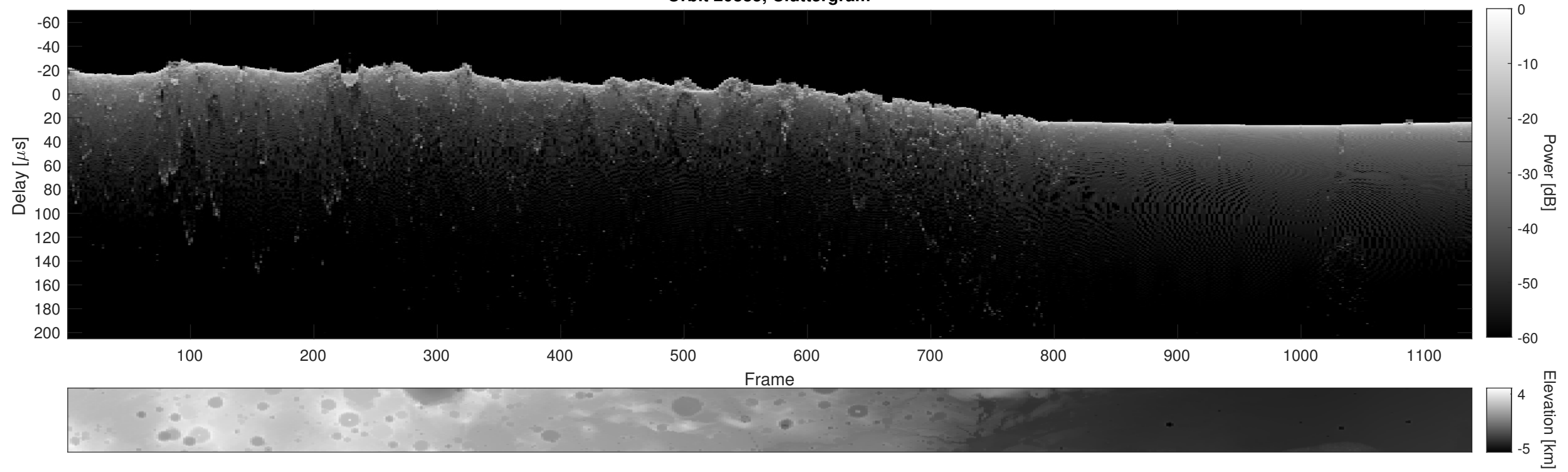
Orbit 20885, Cluttergram
