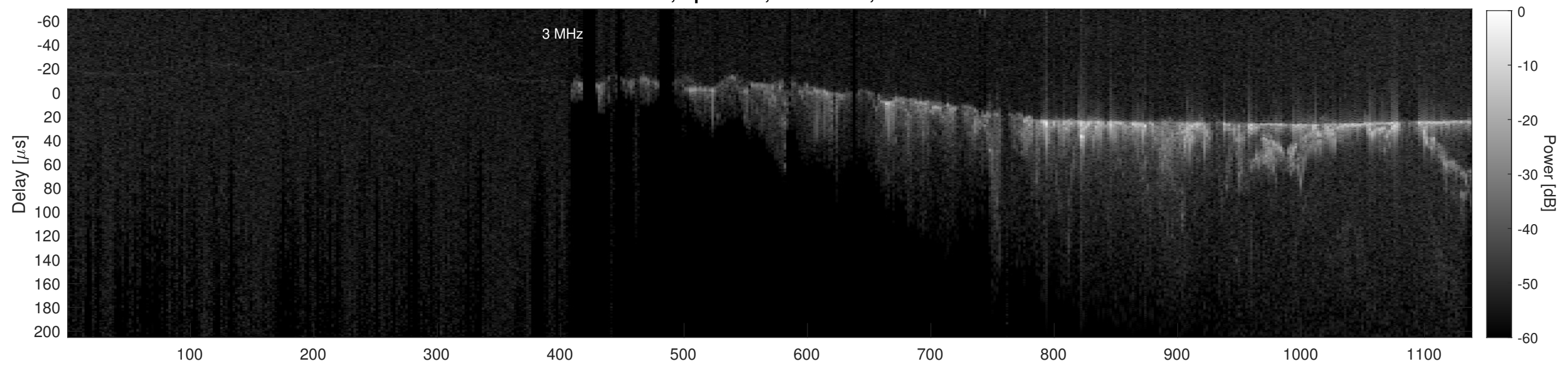
Orbit 20885, Cluttergram
