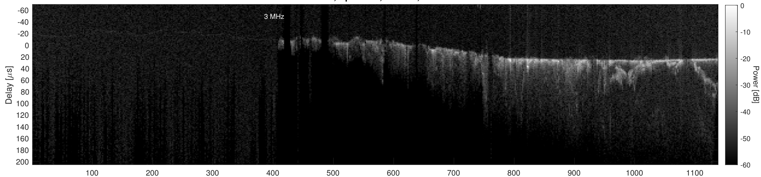
Orbit 20885, Cluttergram
