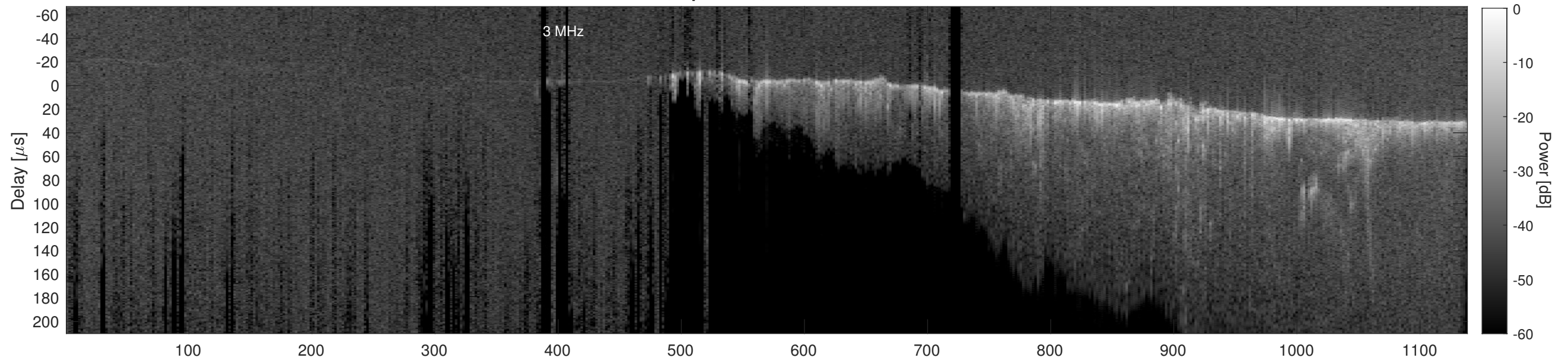
Orbit 20886, Cluttergram
