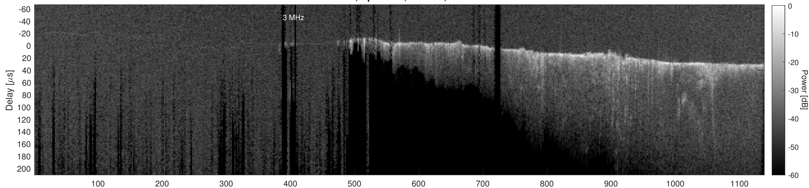
Orbit 20886, Cluttergram
