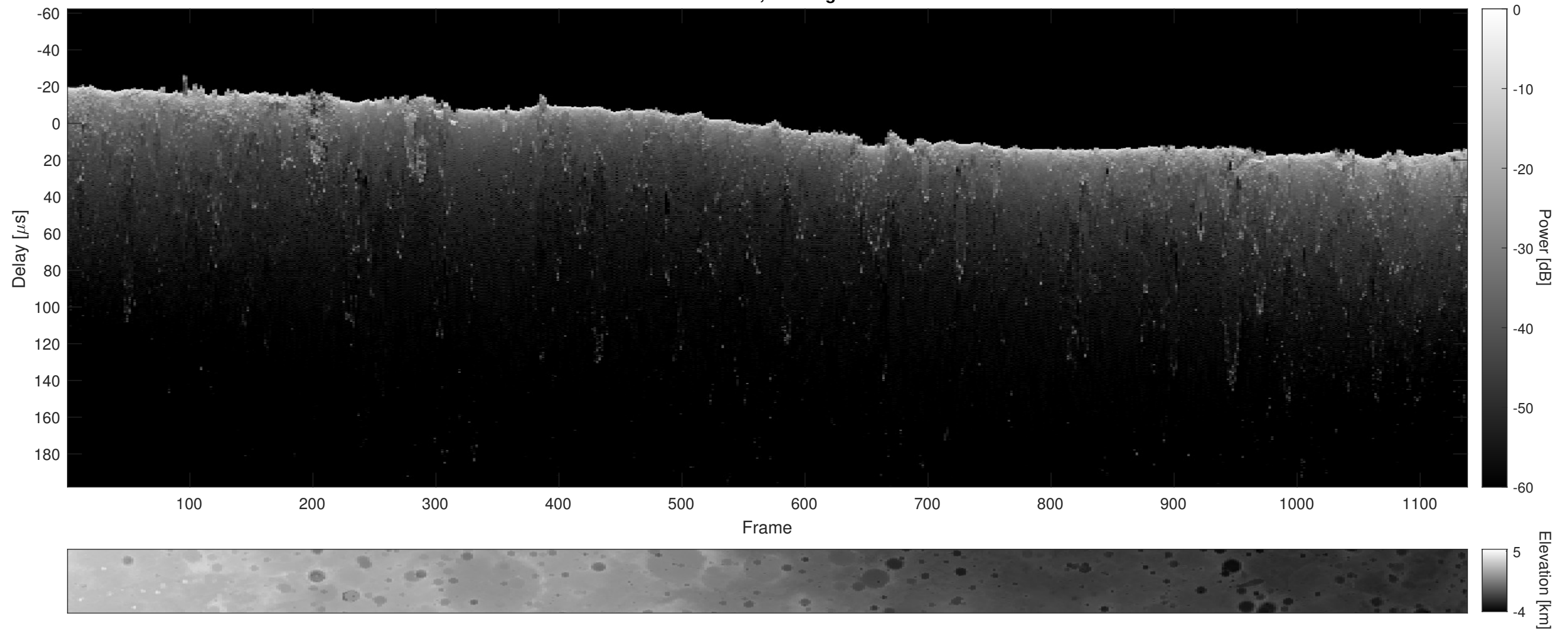
Orbit 20887, Cluttergram
