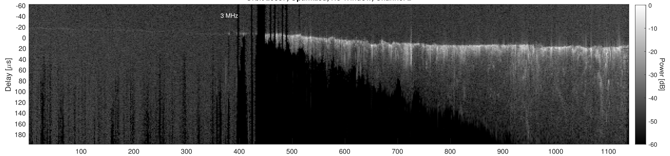
Orbit 20887, Cluttergram
