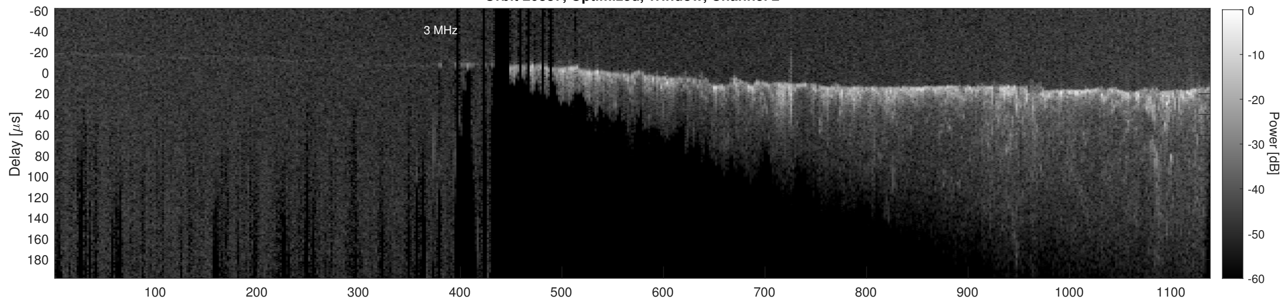
Orbit 20887, Cluttergram
